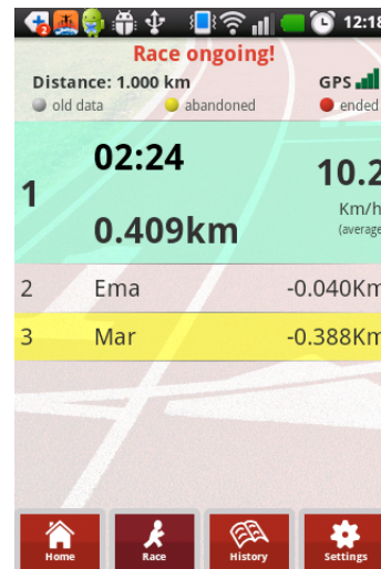
Figure 5. Ongoing race
