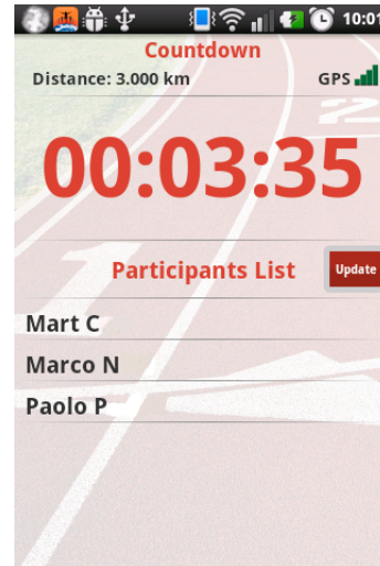
Figure 4. Countdown dialog
