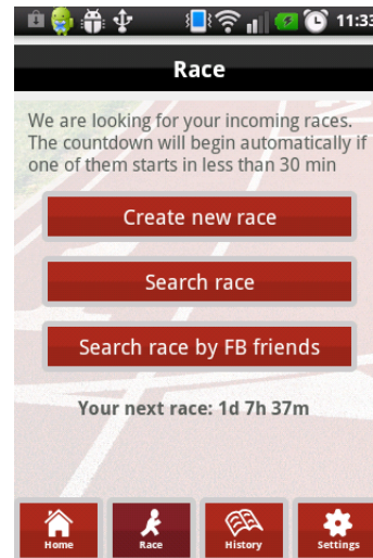
Figure 1. Main menu
