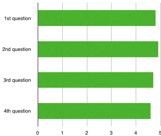
Figure 8. Questionnaire results
