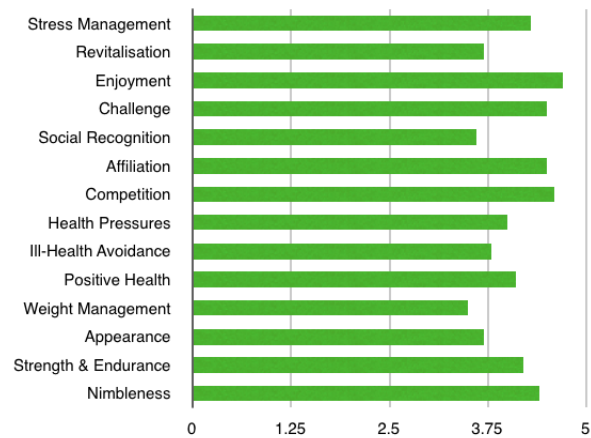
Figure 7. EMI-2 results
