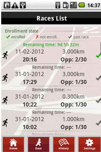
Figure 3. Search results
