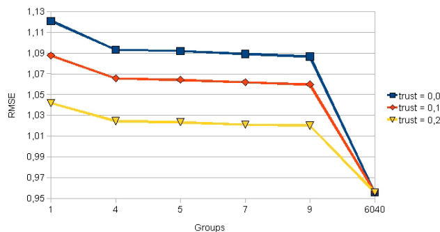
Fig. 3. Algorithm's performances with different trust values
