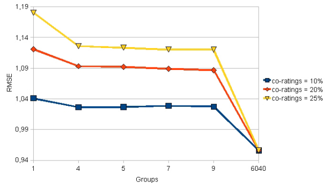
Fig. 2. Algorithm’s performances with different co-ratings values
