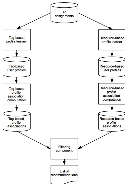
Fig. 1: Architecture of the friend recommender system
